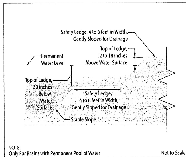
Elevation View - Basin Safety Ledge Configuration
