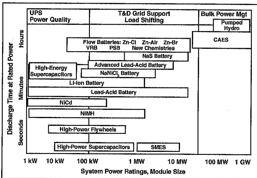
FIGURE D.2(a) Positioning of Energy Storage Technologies. (Source: U.S. Department of Energy, Energy Storage System Guide for Compliance with Safety Codes and Standards.)
