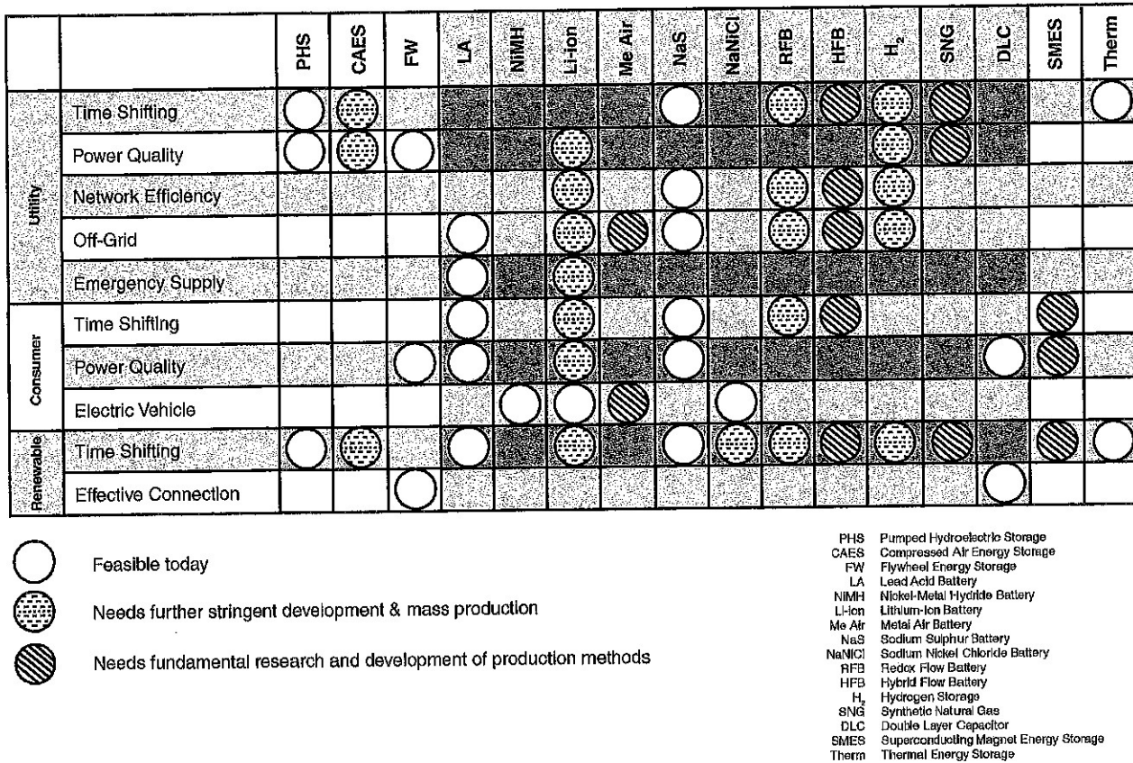
FIGURE D.2(b) ESS Feasibility, Future Potential, and Need for Development by 2030. (Source: Fraunhofer ISE.)
