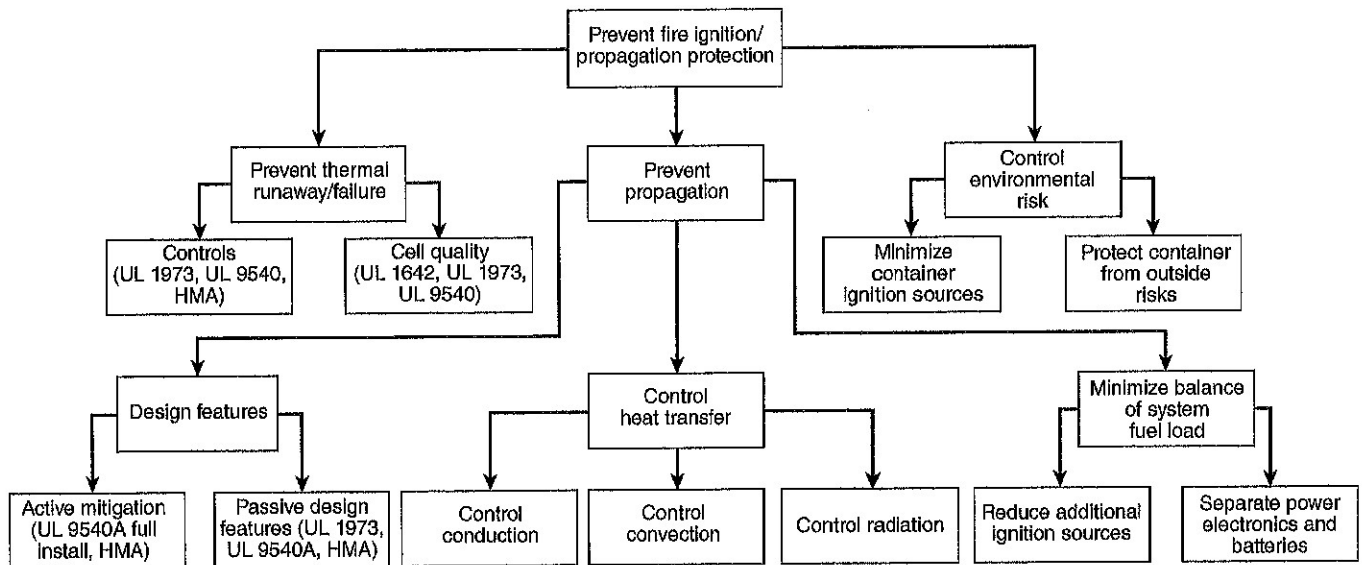
FIGURE G.3.6(c) Example Fire Ignition and Propagation Protection Flow Chart.
