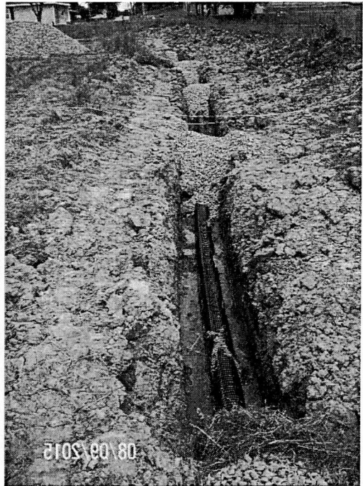
Perforated pipe covered in stone with straw separation layers
