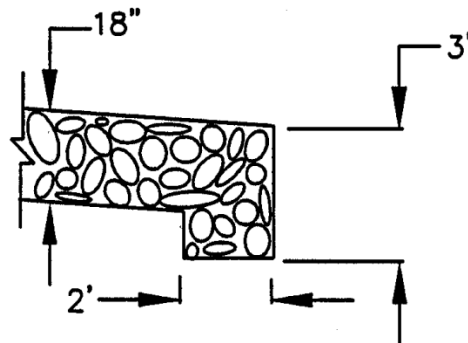
SECTION A-A TOE WALL
