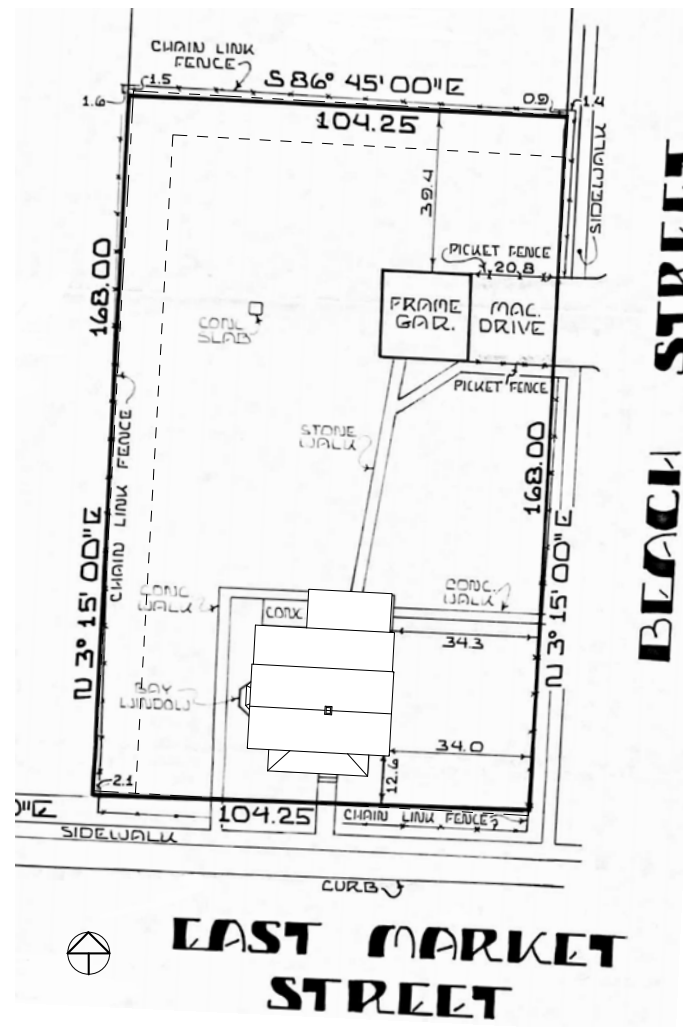
⑨ SITE 1" = 20'-0" SCALE 0 1/2' 1' (ACTUAL) 2'
